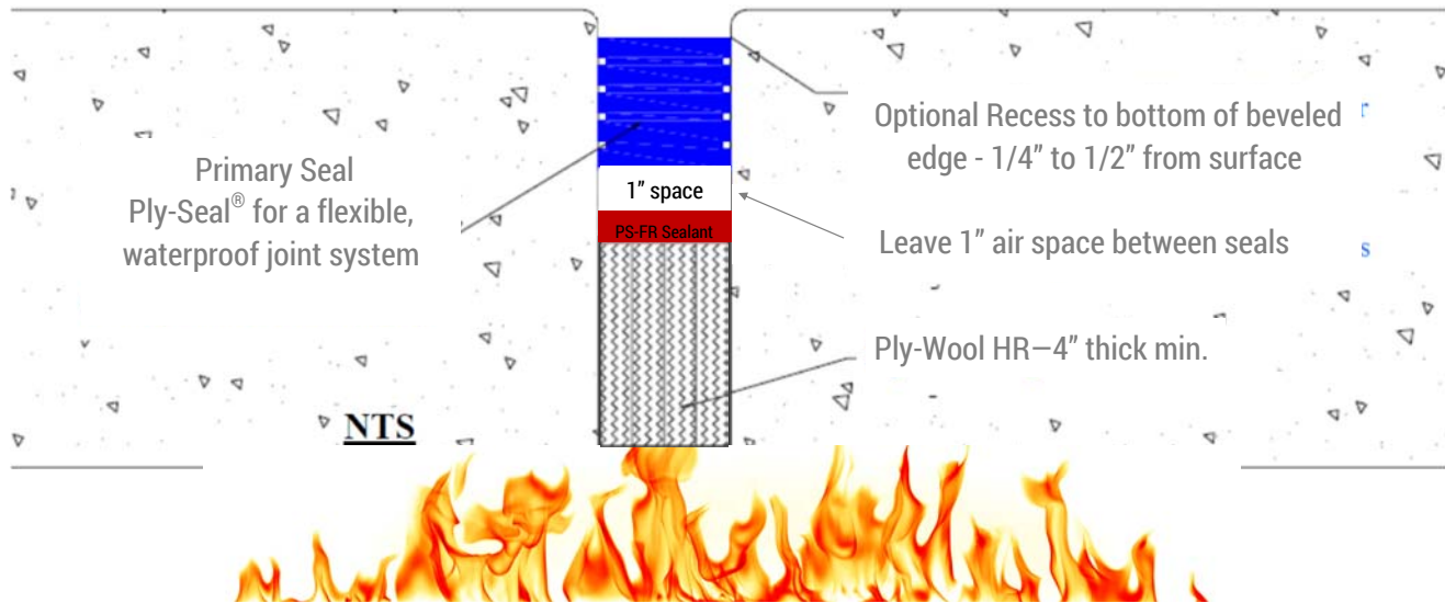
ANSI/UL 2079 System # FF-D-1023 Class II 3 Hr. Fire Stop with Added Waterproof Joint Seal
